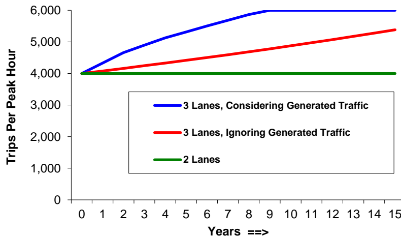
Figure 9 Projected Traffic
